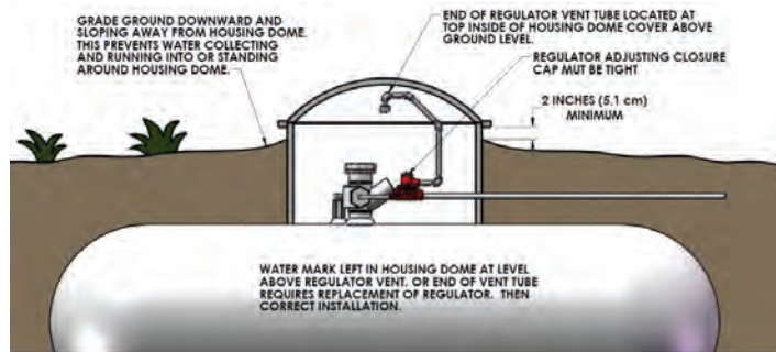
Figure 5: Underground Installation
