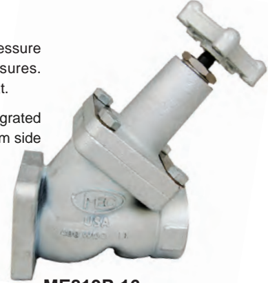
ME819P-16 2" - Flange x NPT Globe Valve
