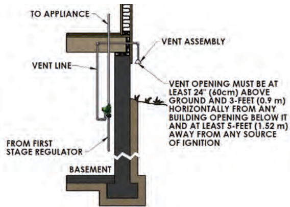
Figure 4: Basement Installation
